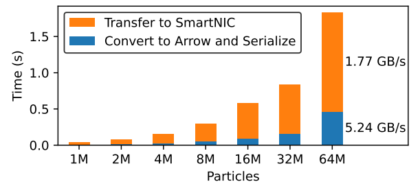
Fig. 6: Data preparation and injection overhead
